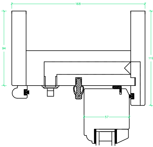
Option to have to Applied Bars.
