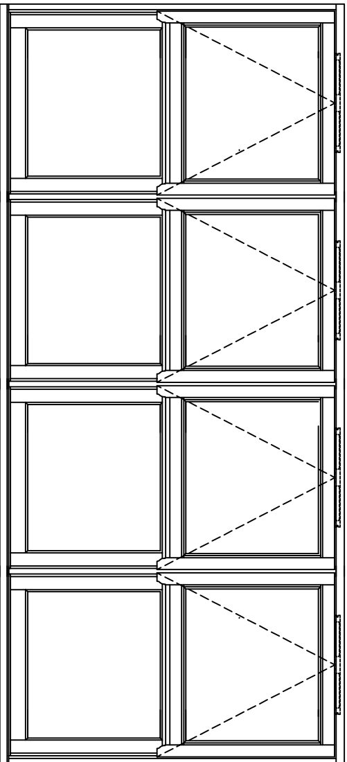
Pseudo Slide Sash Window.
