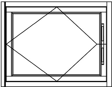
Full Reversible Window
