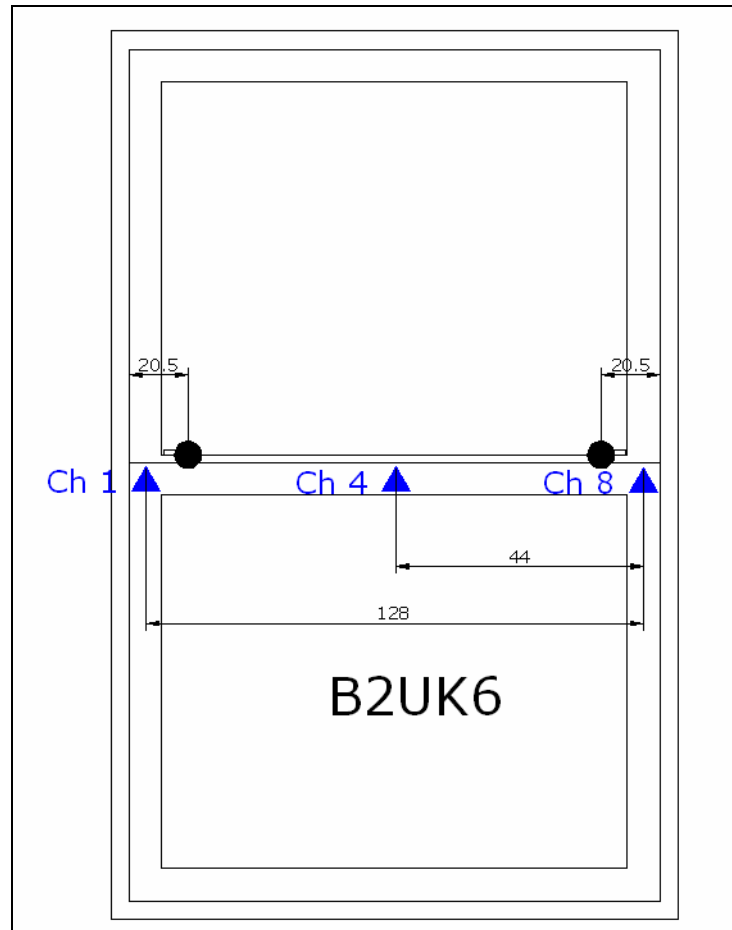
Figure. Location dial gauges (1 - 3)
